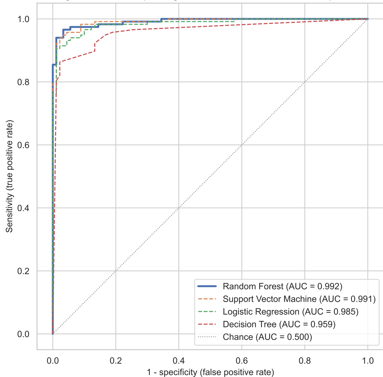
Figure 6. Receiver operating characteristic curves, held-out test partition
